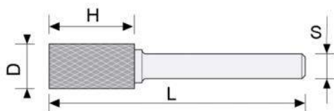
Cilindrcal Shape
